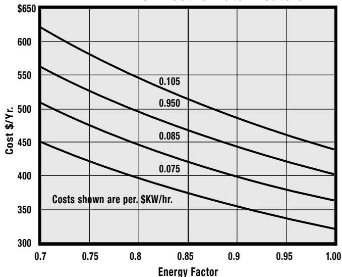
Figure 2 Estimated Annual Operating Cost For Electric Water Heaters
